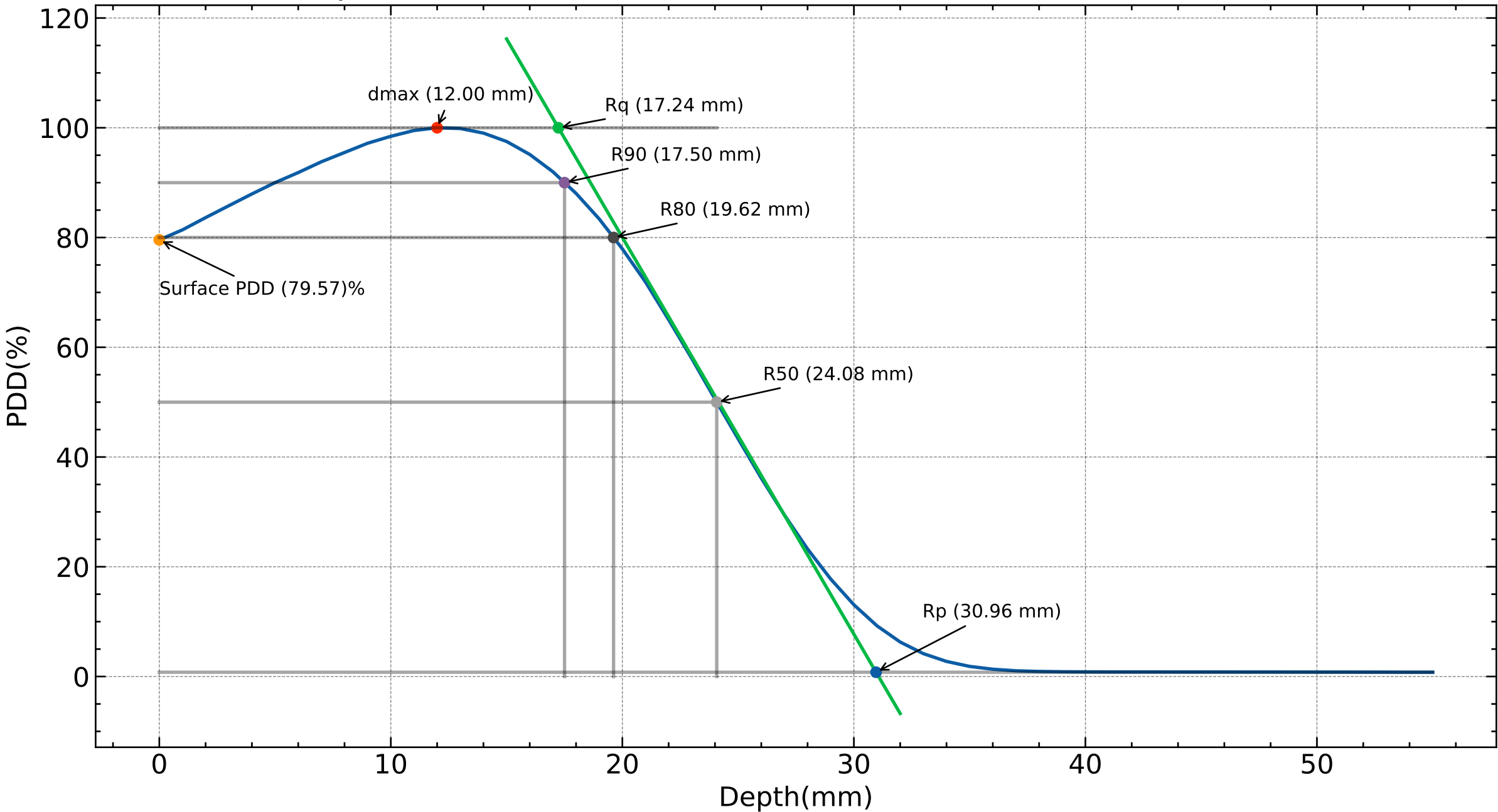
PDD profile of 6 MeV SSD=100, Water Phantom, F.S= 10x10cm 2
